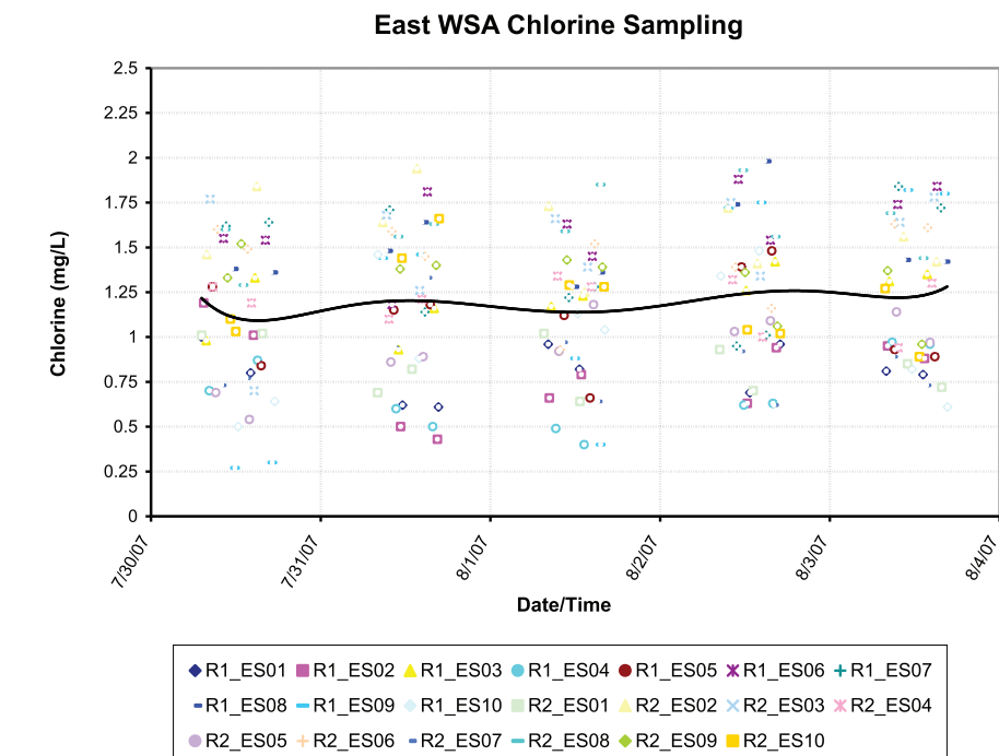
Figure 3: Example Field Chlorine Sampling Results
